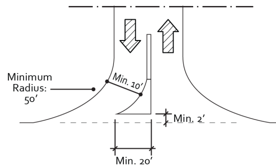
Figure 6-13: Right-in, Right-out, Left-out Driveway Design
